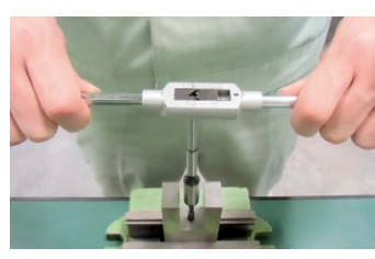
Hand drilling
