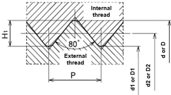
Pg thread form of a German conduit pipe thread (DIN 40430)
