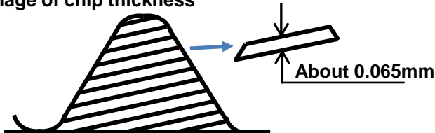
Image of chip thickness
