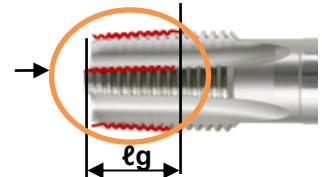
Drawing-2 Cutting portion of a tap for taper pipe threads
