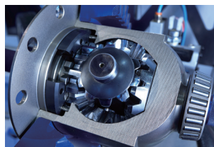
Differential gear
