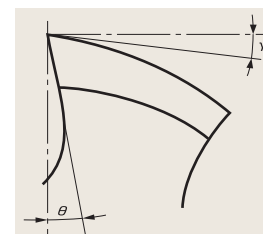
Rake angle (θ:Cutting angle, γ:Chamfer relief angle)
